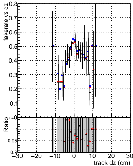
Fake rate vs dz —●— DGM mkFit TT base —●— DGM mkFit TT retrain —●— DGM mkFit TT retrain —●— DGM mkFit TT noCandDNN
