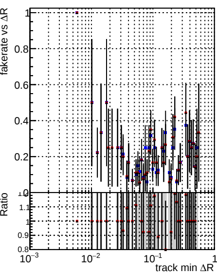
Fake rate vs \Delta R(\text{track, jet}) Legend: DQM_mkFit_TT_base (blue circles) DQM_mkFit_TT_retrain_noCandDNN (red circles) DQM_mkFit_TT_retrain (black circles)
