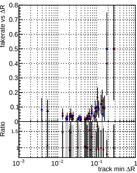
Fake rate vs \Delta R(\text{track}, \text{jet}) Legend: DQM_mkFit_TT_base (blue) DQM_mkFit_TT_retrain_noCandDNN (red) DQM_mkFit_TT_retrain (black)
