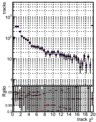
N of reco track vs. s DQM mkFit base mkFit retrain noCandDNN mkFit retrain
