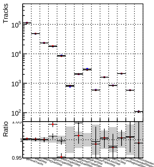
Number of tracks vs collection Legend: DQM_mkFit_TT_base DQM_mkFit_TT_retrain_noCandDNN DQM_mkFit_TT_retrain
