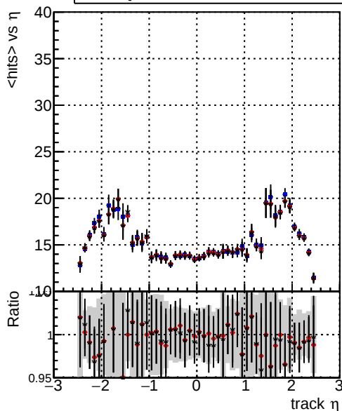
mean hit — DQM_mkFit_TT_base — DQM_mkFit_TT_retrain_noCandDNN — DQM_mkFit_TT_retrain
