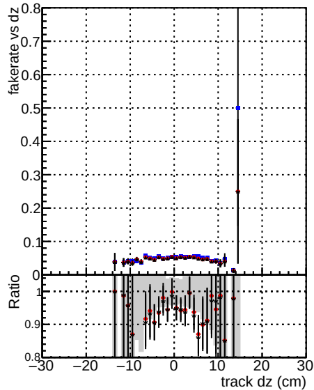
— DOM mkFit TT base — DOM mkFit TT retrain — DOM mkFit TT noCandDNN
