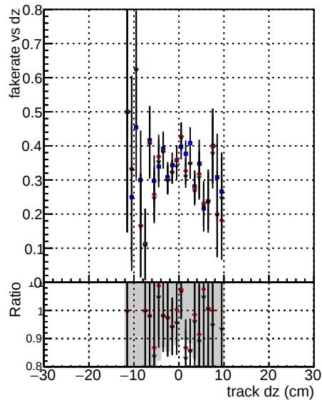
Fake rate vs dz —●— DOM mkFit TT base —●— DOM mkFit TT retrain — noCandDNN
