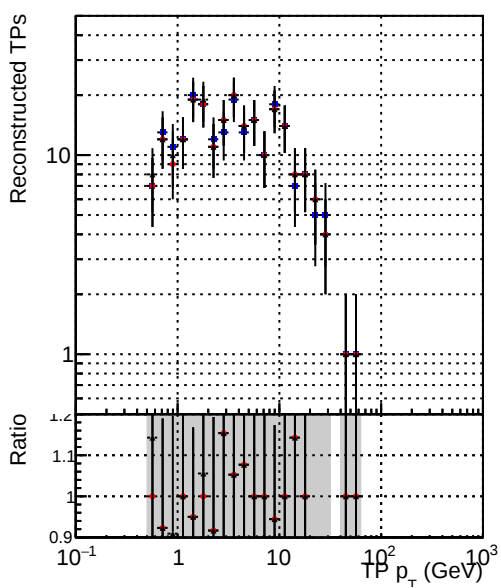
Legend: —•— DQM_mkFit_TT_base —•— DQM_mkFit_TT_retrain_noCandDNN —•— DQM_mkFit_TT_retrain
