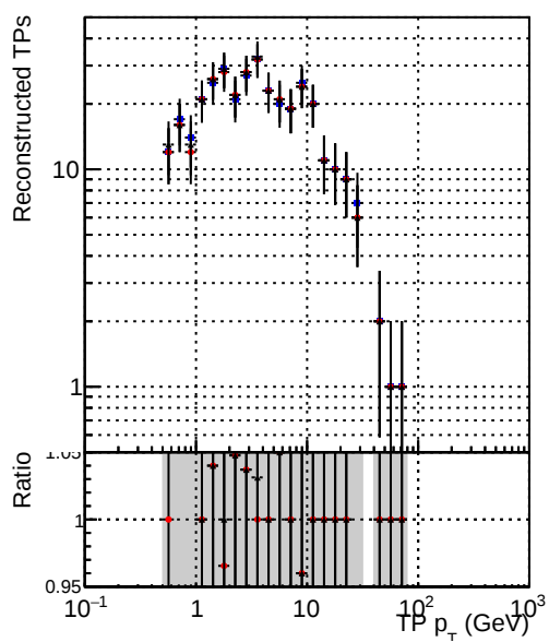
Legend: DQM_mkFit_TT_base (Blue line with circles) DQM_mkFit_TT_retrain_noCandDNN (Red line with circles) DQM_mkFit_TT_retrain (Black line with circles)
