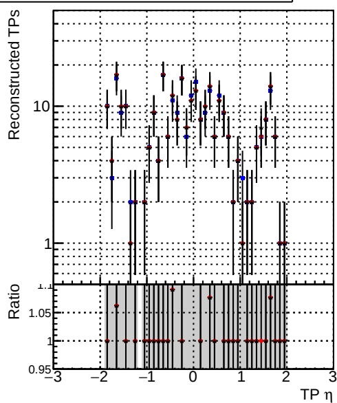
Legend: DQM_mkFit_TT_base (Blue line with circles) DQM_mkFit_TT_retrain_noCandDNN (Red line with circles) DQM_mkFit_TT_retrain (Black line with circles)
