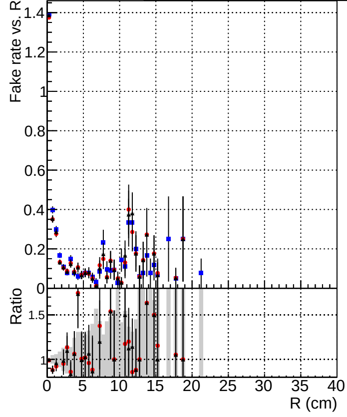
K_S^0 tracking fake rate vs R Legend: DQM_mkFit_TT_base (blue squares) DQM_mkFit_TT_retrain_noCandDNN (red circles) DQM_mkFit_TT_retrain (black triangles)
