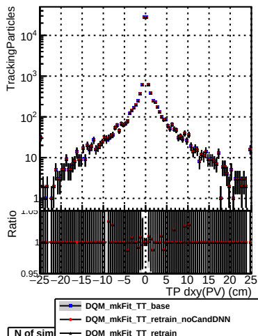
N of sim → DQM_mkFit_TT_retrain
