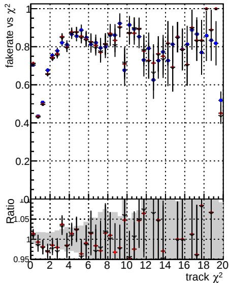
Fake rate vs. DOM mkFit TT base DOM mkFit TT retrain DOM mkFit TT retrain noCandDNN
