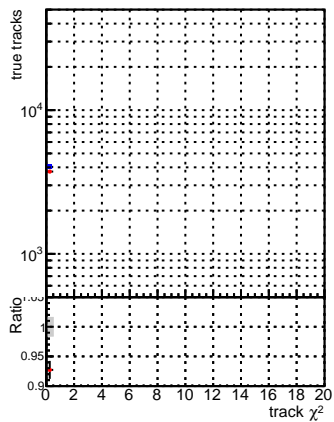
Legend: - Blue line: DQM_CKF_QCDHighPt_retrain - Red line: DQM_mkFit_QCDHighPt_retrain - Grey shaded area: OverSet
