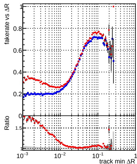
— DQM_CKF_QCDHighPt_retrain — DQM_mkFit_QCDHighPt_retrain
