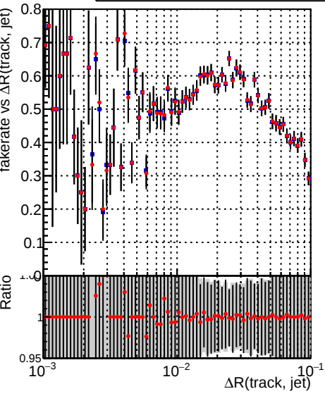
Legend: \blacksquare DQM_CKF_QCDHighPt_retrain \bullet DQM_mkFit_QCDHighPt_retrain
