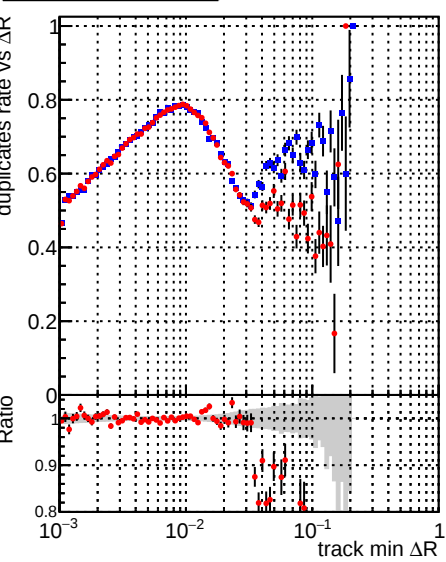
Legend: \blacksquare DQM_CKF_QCDHighPt_retrain \bullet DQM_mkFit_QCDHighPt_retrain
