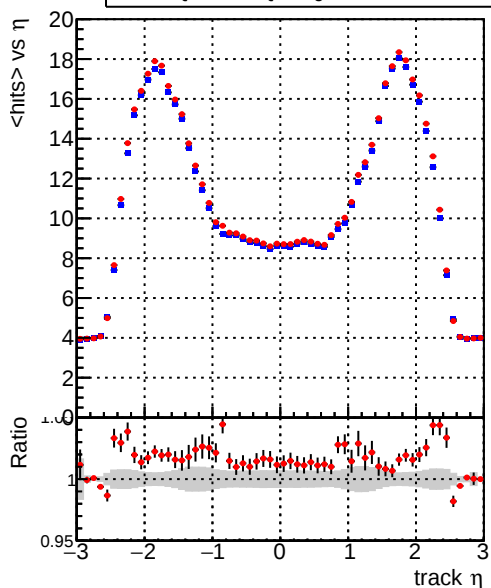
— DQM_CKF_QCDHighPt_retrain — DQM_mkFit_QCDHighPt_retrain
