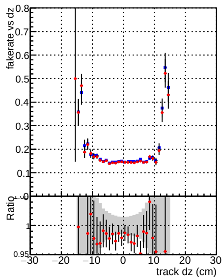
—●— DQM_CKFit_QCDHighPt_retrain —●— DQM_mkFit_QCDHighPt_retrain
