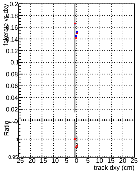
—●— DQM_CKFit_QCDHighPt_retrain —●— DQM_mkFit_QCDHighPt_retrain
