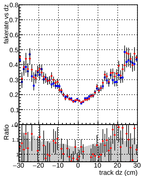
Fake rate vs dz —●— DQM_CKF_QCDHighPt_retrain —●— DQM_mkFit_QCDHighPt_retrain
