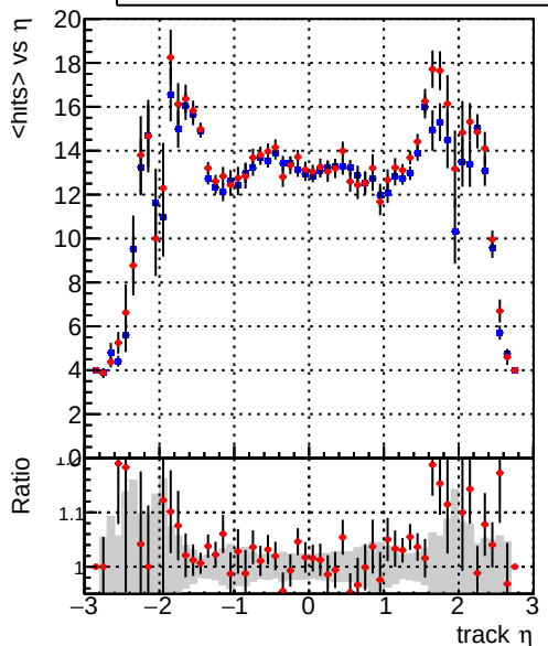
mean hits vs \eta Legend: DQM_CKF_QCDHighPt_retrain (blue line), DQM_mkFit_QCDHighPt_retrain (red line)
