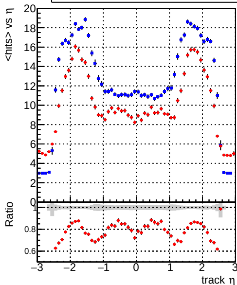
mean hits — DQM_CKF_QCDHighPt_retrain — DQM_mkFit_QCDHighPt_retrain
