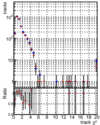
N of reco track vs. \chi^2 DQM_CKF_QCDHighPt_retrain DQM_mkFit_QCDHighPt_retrain
