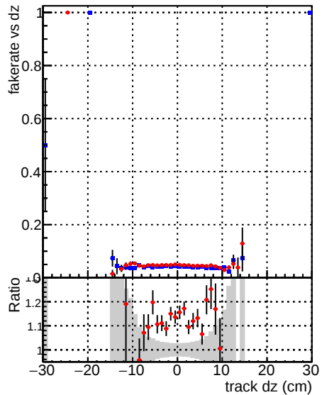
—●— DQM_CKF_QCDHighPt_retrain —●— DQM_mkFit_QCDHighPt_retrain
