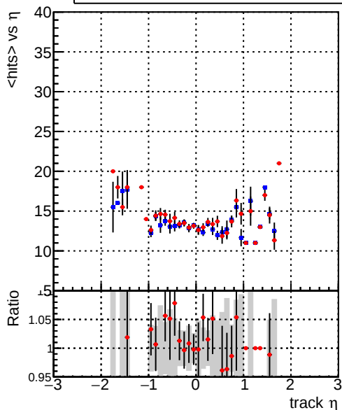
mean hits Legend: — DQM_CKF_QCDHighPt_retrain, — DQM_mkFit_QCDHighPt_retrain
