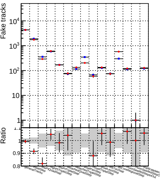
Number —●— DQM_mkFit_QCDHighPt_retrain
