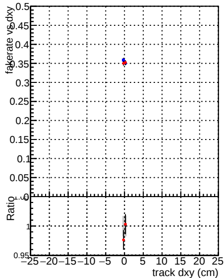
—●— DQM_CKF_QCDHighPt_retrain —●— DQM_mkFit_QCDHighPt_retrain
