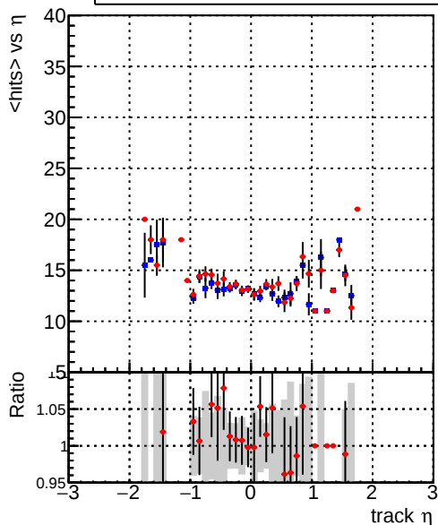
mean hits vs \eta Legend: DQM_CKF_QCDHighPt_retrain (blue line), DQM_mkFit_QCDHighPt_retrain (red line)
