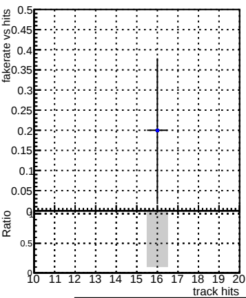
Fake rate vs hit — DQM_CKF_QCDHighPt_retrain — DQM_mkFit_QCDHighPt_retrain
