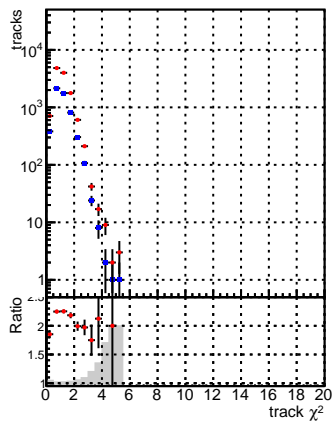
DQM_CKF_QCDHighPt_retrain DQM_mkFit_QCDHighPt_retrain
