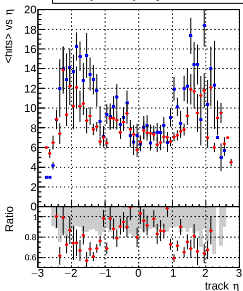
— DQM_CKF_QCDHighPt_retrain — DQM_mkFit_QCDHighPt_retrain mean hit
