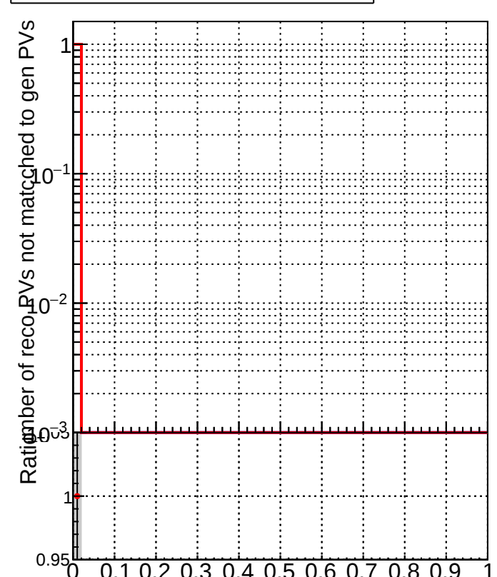
RecoPVAssoc2GenPVNotMatched_Purity
