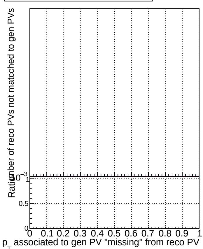
RecoPVAssoc2GenPVNotMatched_missing
