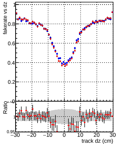
—●— DQM_CKF_QCDHighPt_retrain —●— DQM_mkFit_QCDHighPt_retrain
