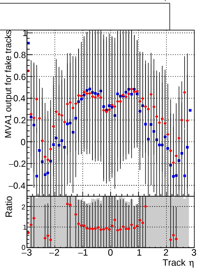
MVA1 of associated tracks (recoToSim) vs. Track \eta Legend: ■ DQM_CKF_QCDHighPt_retrain ● DQM_mkFit_QCDHighPt_retrain
