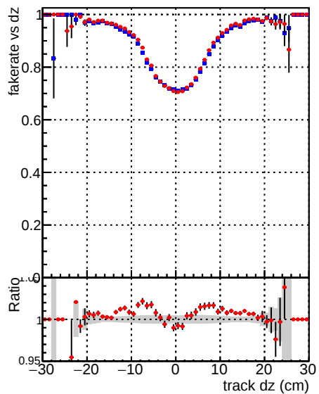
—●— DQM_CKF_QCDHighPt_retrain —●— DQM_mkFit_QCDHighPt_retrain
