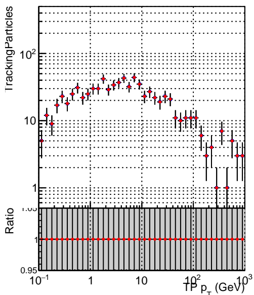
—●— DQM_CKF_QCDHighPt_retrain —●— DQM_mkFit_QCDHighPt_retrain
