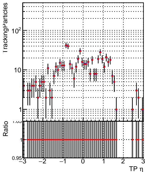
—●— DQM_CKF_QCDHighPt_retrain —●— DQM_mkFit_QCDHighPt_retrain
