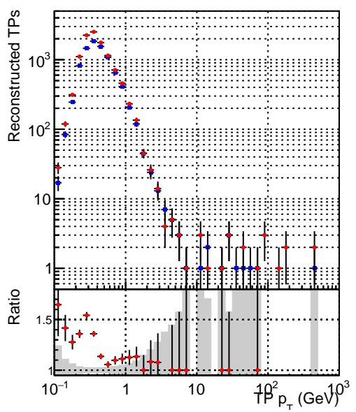
■ DQM_CKF_QCDHighPt_retrain ● DQM_mkFit_QCDHighPt_retrain
