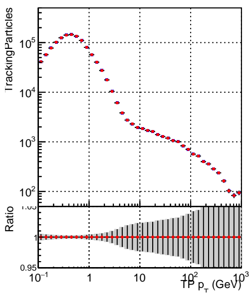
■ DQM_CKF_QCDHighPt_retrain ● DQM_mkFit_QCDHighPt_retrain
