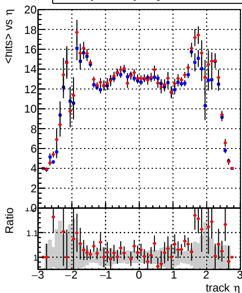
mean hits vs \eta — DQM_CKF_QCDHighPt_retrain — DQM_mkFit_QCDHighPt_retrain
