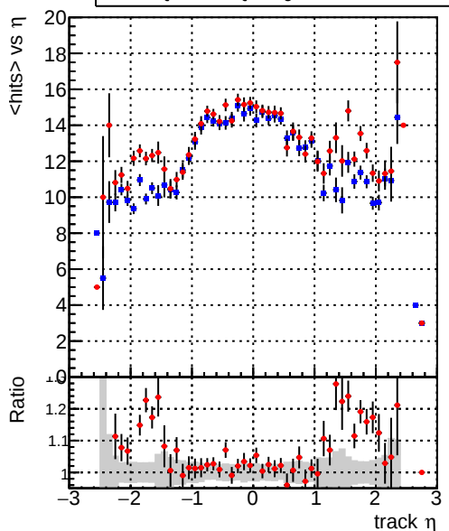
mean hit — DQM_CKF_QCDHighPt_retrain — DQM_mkFit_QCDHighPt_retrain
