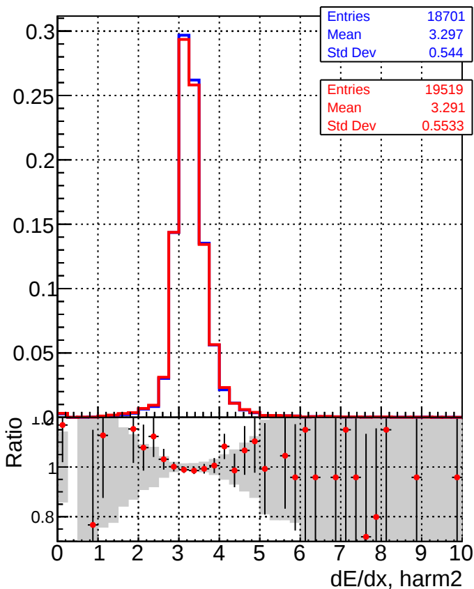
DQM_CKF_QCDHighPt_retrain DQM_mkFit_QCDHighPt_retrain
