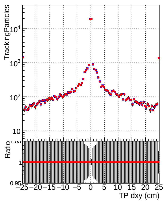
N of simulated track Legend: DQM_CKF_QCDHighPt_base DQM_mkFit_QCDHighPt_base
