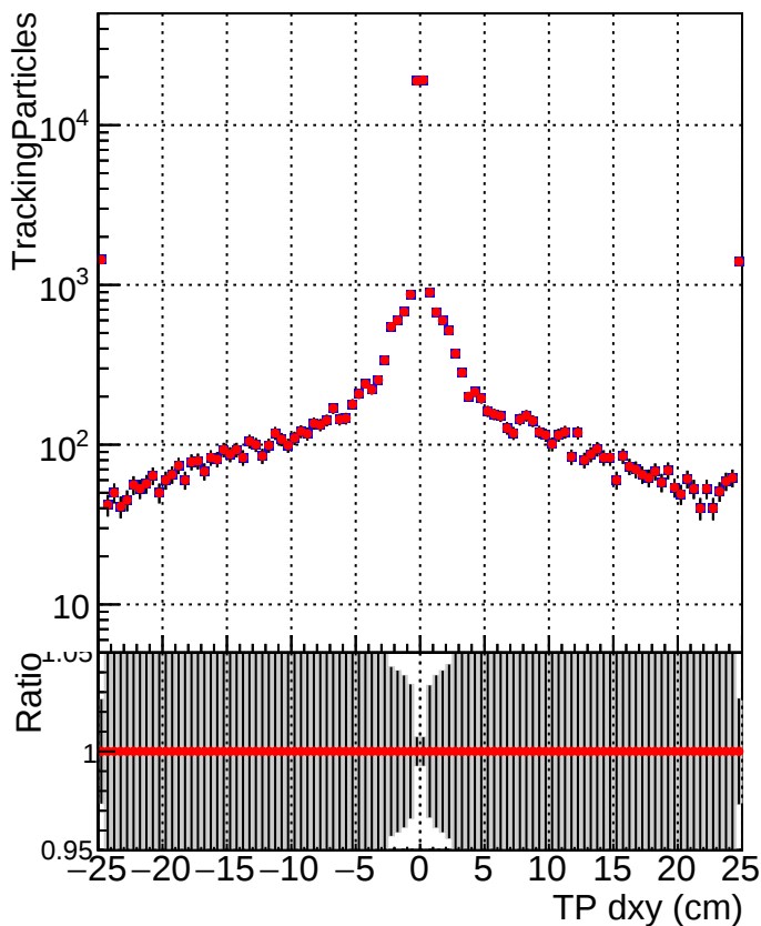
■ DQM_CKF_QCDHighPt_base ■ DQM_mkFit_QCDHighPt_base
