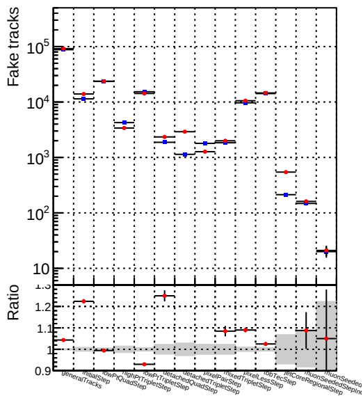
Number —●— DQM_mkFit_QCDHighPt_base
