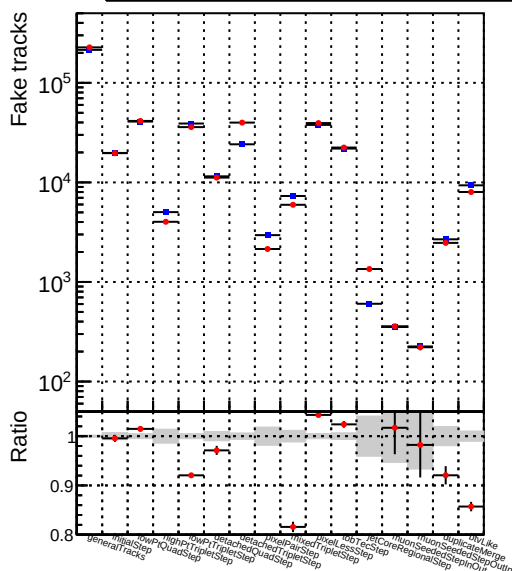
Number —●— DOM mkFit OCDHighPt base
