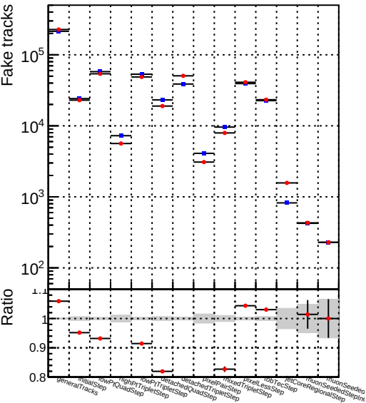
Number —●— DQM_mkFit_QCDHighPt_base
