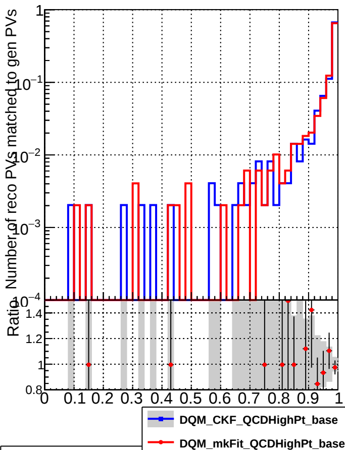
RecoPVAssoc2GenPVMatched_missing
