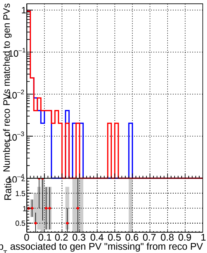
RecoPVAssoc2GenPVMatched_missing
