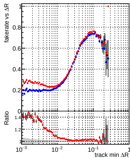
—♦— DQM_CKF_QCDHighPt_base —♦— DQM_mkFit_QCDHighPt_base
