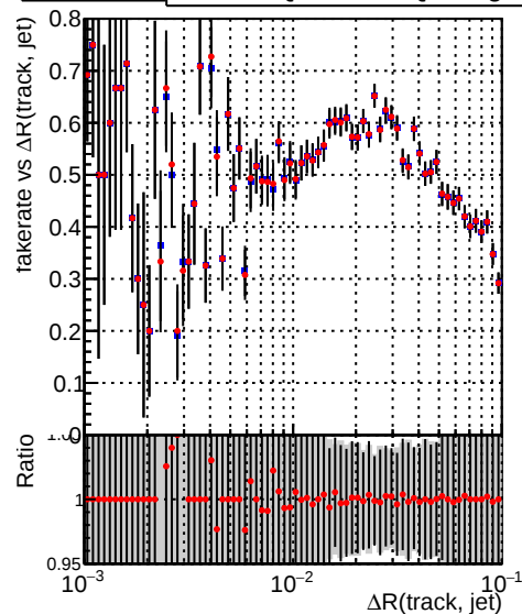
Fake rate vs \Delta R(\text{track, jet}) Legend: —•— DQM_CKF_QCDHighPt_base —•— DQM_mkFit_QCDHighPt_base
