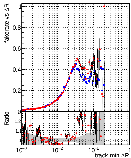
Fake rate vs \Delta R(\text{track, jet}) Legend: —•— DQM_CKF_QCDHighPt_base —•— DQM_mkFit_QCDHighPt_base
