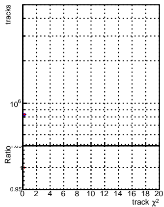
Legend: DQM_CKF_QCDHighPt_base DQM_mkFit_QCDHighPt_base
