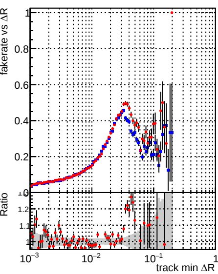
Fake rate vs \Delta R (track, jet) DQM_CKF_QCDHighPt_base DQM_mkFit_QCDHighPt_base
