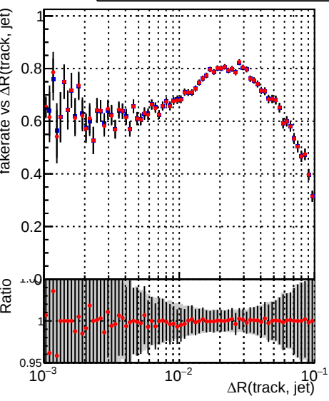
Fake rate vs \Delta R (track, jet) DQM_CKF_QCDHighPt_base DQM_mkFit_QCDHighPt_base
