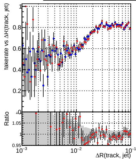
—•— DQM_CKF_QCDHighPt_base —•— DQM_mkFit_QCDHighPt_base
